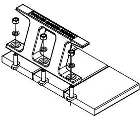
CLEAT SSEMBLY DETAIL
