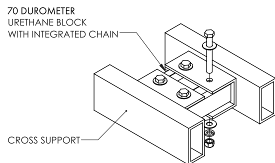
TYPICAL DOCK TO DOCK CONNECTION
