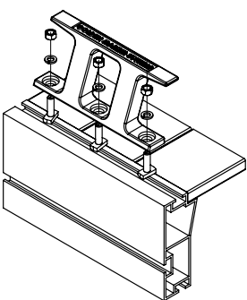
CLEAT ASSEMBLY DETAIL
