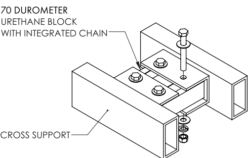
TYPICAL DOCK TO DOCK CONNECTION
