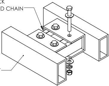
TYPICAL DOCK TO DOCK CONNECTION
